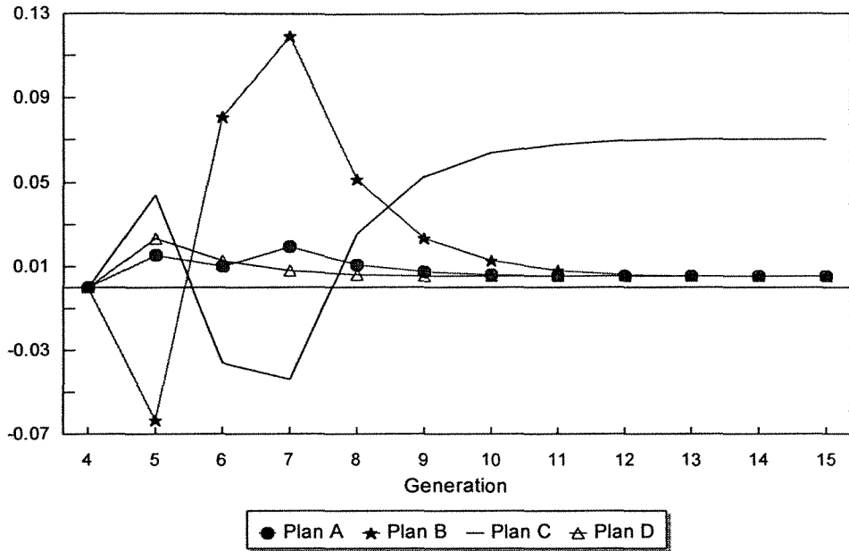
Figure 1a Lifetime Utility Eliminating the Social Security Tax Difference from Baseline \eta = .1
