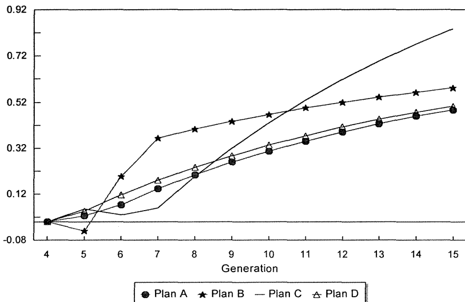
Figure 1b Lifetime Utility Eliminating the Social Security Tax Difference from Baseline \eta = .6
